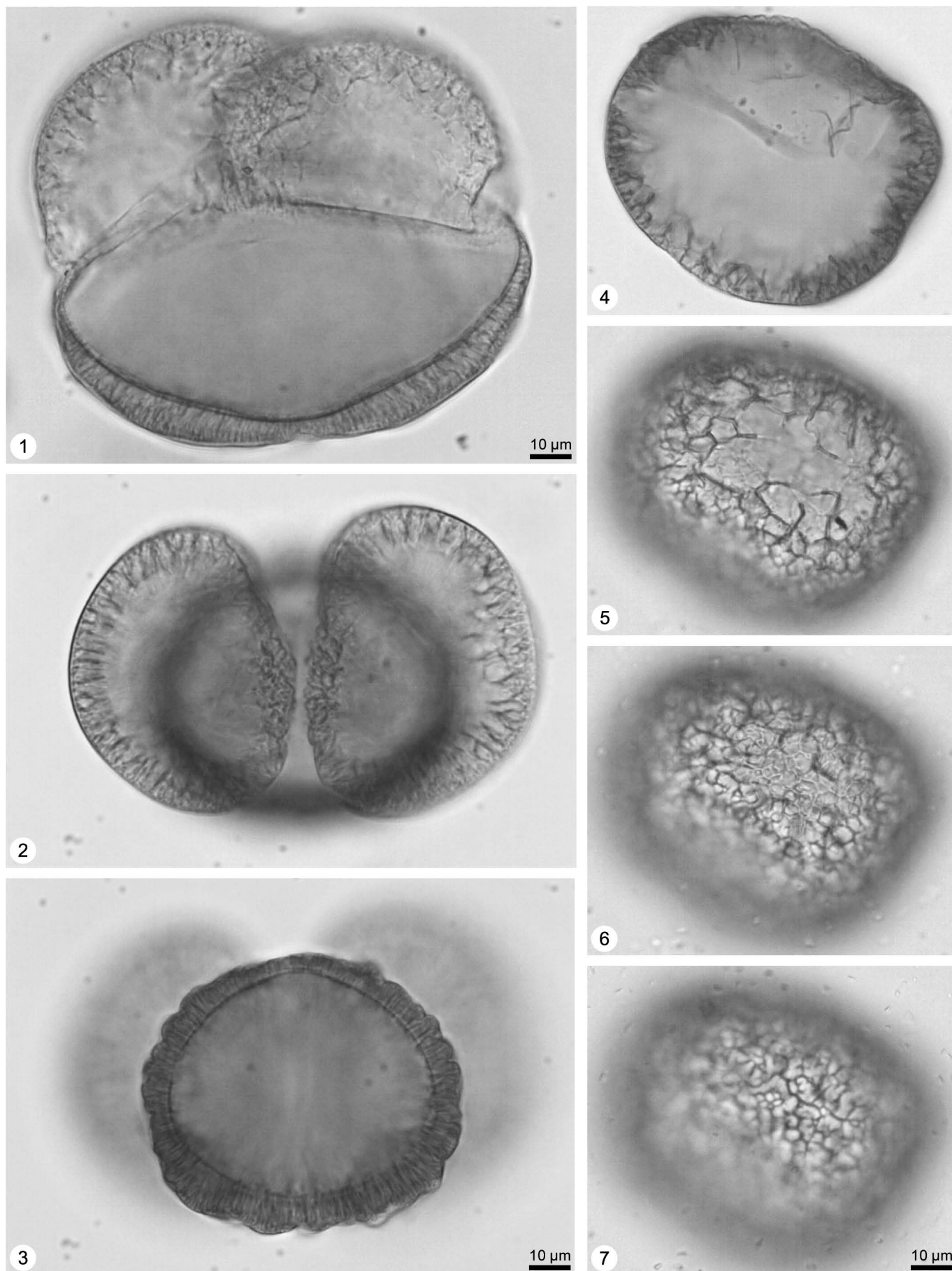
Plate III. Lake Suigetsu Pollen Flora: Coniferopsida. Pinaceae: 1 Abies (lateral view), 2-3 Abies (view on distal face, high and low focus), 4-7 Abies , detached air-sack (view through ruptured attachment zone, from high to low focus). Photos/imaging: D. Demske, FUB.
