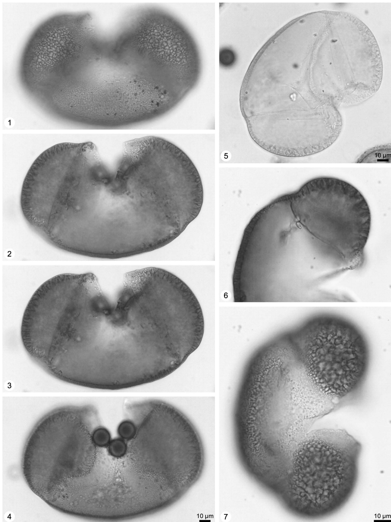
Plate V. Lake Suigetsu Pollen Flora: Coniferopsida. Pinaceae: 1-4 Picea sect. Eupicea type (lateral view, from high to low focus, lower magnification), 5 Picea sect. Eupicea type (oblique lateral view, lower magnification), 6-7 Picea sect. Omorika type (lateral view, high and low focus). Photos/imaging: D. Demske, FUB.
