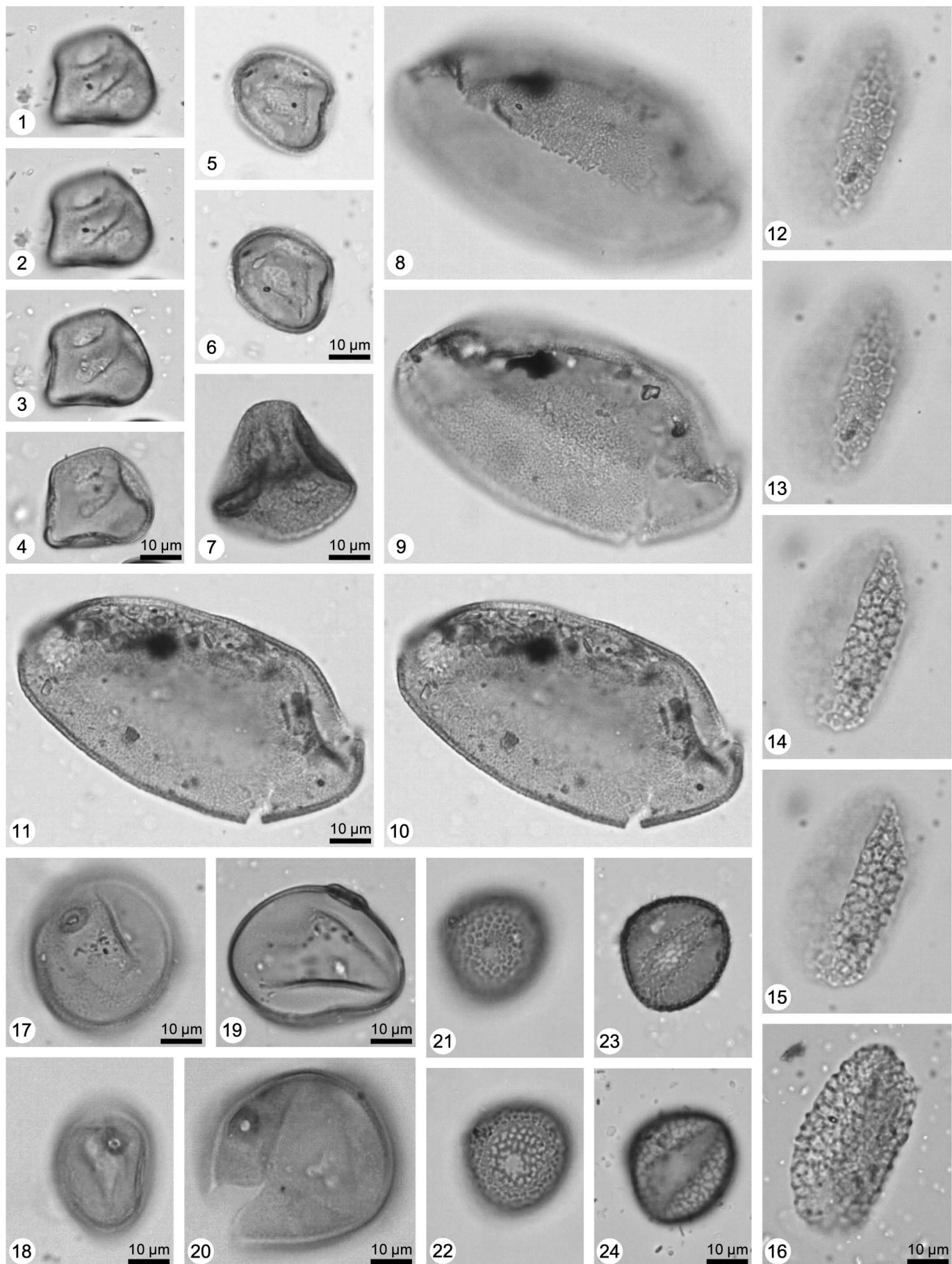
Plate XVI. Lake Suigetsu Pollen Flora: Magnoliopsida - Liliidae (monocots). Cyperaceae: 1-4, 5-6 Cyperus type (equatorial view, from high to low focus), 7 Rhynchospora type (crumpled grain). Iridaceae: 8-11 Iridaceae, cf. Iris humilis type, 12-16 Iris type (8-16, oblique view, 8-11, 12-16 from high to low focus). Poaceae: 17, 18 Poaceae undiff., 19 Poaceae cereal type, 20 Poaceae wildgrass type (size > 40 µm, non-cereal anulus). Typhaceae (incl. Sparganiaceae): 21-24 Sparganium (view on distal face, from high to low focus). Photos/imaging: D. Demske, FUB.
