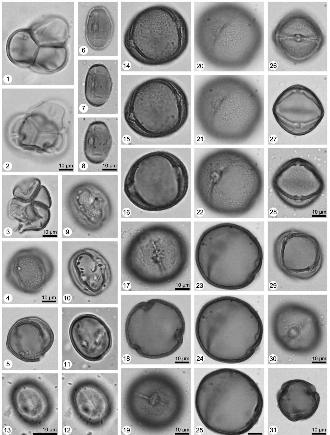
Plate XXVI. Lake Suigetsu Pollen Flora: Magnoliopsida - Rosidae (eudicots). Ericaceae: 1-2 Ericaceae undiff., 3 Pyrola type (tetrads, 1-2 high and low focus). Euphorbiaceae: 4-5 Euphorbia type (4-5 equatorial view, high to low focus). Fabaceae: 6-8 Fabaceae undiff., 9-13 Astragalus/Oxytropis type (6-13 equatorial view, 6-8, 9-13 high to low focus). Fagaceae: 14-17, 18, 19, 20-25 Fagus crenata type, 26-28, 29-30, 31 Fagus japonica type (14-17, 19-30 equatorial view, 18, 31 polar view, 14-17, 20-25, 26-28, 29-30 high to low focus). Photos/imaging: D. Demske, FUB.
