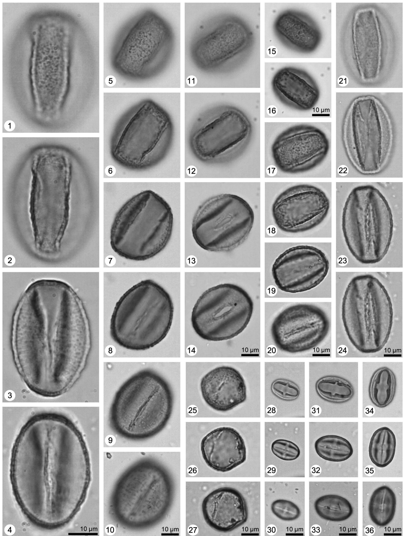
Plate XXVIII. Lake Suigetsu Pollen Flora: Magnoliopsida - Rosidae (eudicots). Fagaceae (deciduous oaks): 1-4 Quercus subgen. Lepidobalanus type (higher magnification), 5-10, 11-14, 15-16, 17-20, 21-24 Quercus subgen. Ledpidobalanus type (1-24 equatorial view, 1-4, 5-10, 11-14, 15-16, 17-20, 21-24 from high to low focus). Fagaceae (other): 25-27 Quercus undiff., 28-30, 31-33, 34-36 Castanea/Castanopsis type (25-36 equatorial view, 25-27, 28-30, 31-33, 34-36 from high to low focus). Photos/imaging: D. Demske, FUB.
