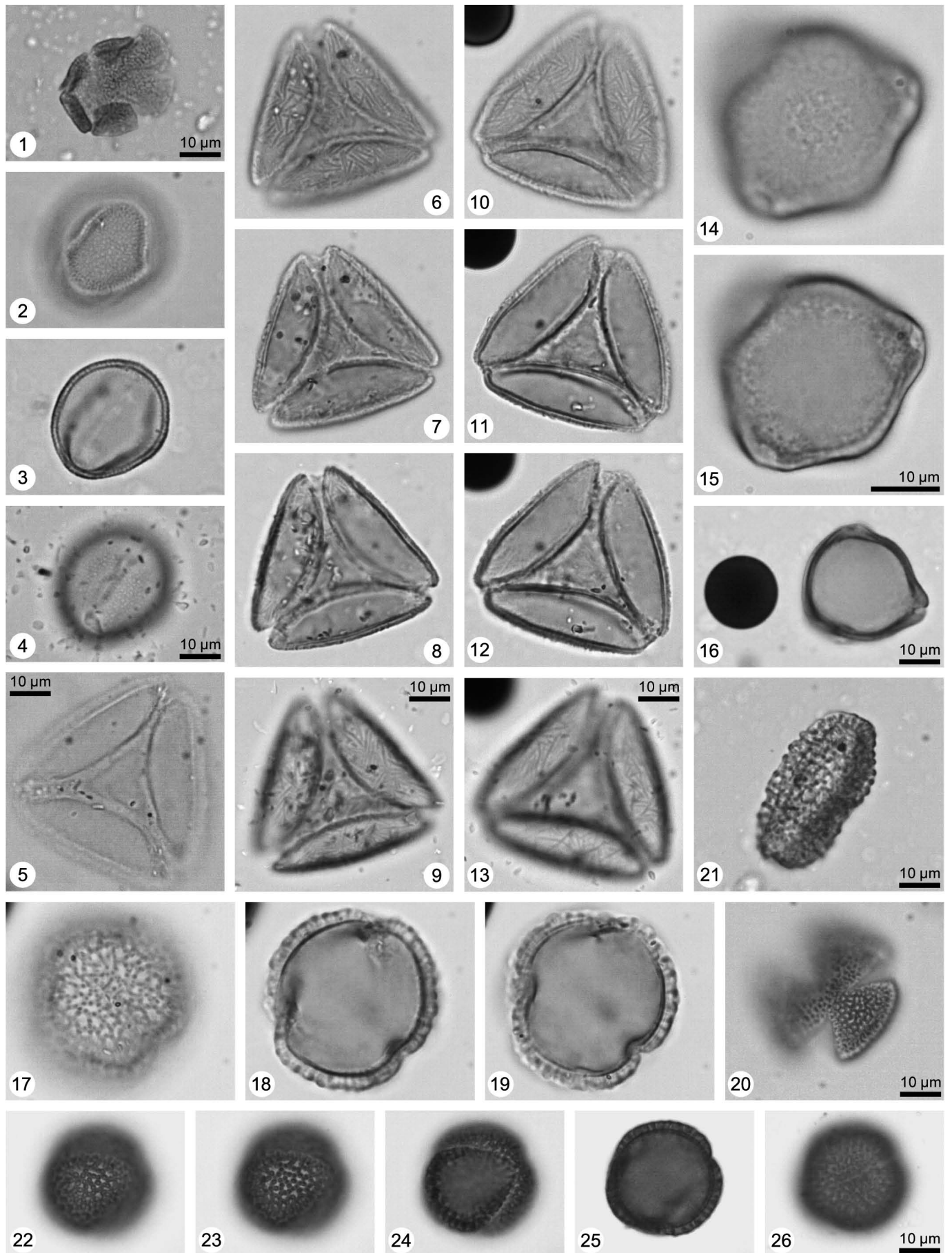
Plate XXX. Lake Suigetsu Pollen Flora: Magnoliopsida - Rosidae (eudicots). Lamiaceae: 1 Prunella type (polar view), 2-4 Stachys type (equatorial view, high to low focus); Menyanthaceae: 5, 6-9, 10-13 Nymphoides (5 degraded, 5-13 polar view, 6-9, 10-13 high to low focus). Myricaceae: 14-15, 16 Myrica (14-16 polar view, 14-15 high to low focus, higher magnific., 16 with 15 \mu m marker). Oleaceae: 17-19, 20, 21, 22-26 Ligustrum/Syringa (17-20 polar view, 21 equatorial view, 22-26 subpolar view, 17-19, 22-26 high to low focus). Photos/imaging: D. Demske, FUB.
