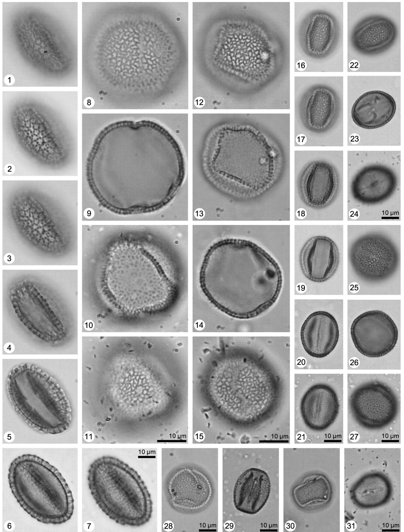
Plate XXXI. Lake Suigetsu Pollen Flora: Magnoliopsida - Rosidae (eudicots). Oleaceae: 1-7 Ligustrum/Syringa (equatorial view, from high to low focus), 8-11, 12-15 Fraxinus (8-11 subpolar view, 12-15 equatorial view, 8-11, 12-15 from high to low focus, higher magnification), 16-21, 22-24, 25-27 Fraxinus , aff. Fraxinus ornus type (16-27 equatorial view, 16-21, 22-24, 25-27 from high to low focus), 28, 29, 30-31 Fraxinus undiff. (28 subpolar view, 29-31 equatorial view, 30-31 from high to low focus). Photos/imaging: D. Demske, FUB.
