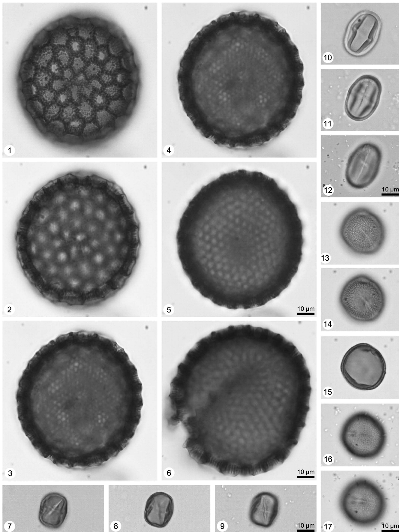
Plate XXXIV. Lake Suigetsu Pollen Flora: Magnoliopsida - Rosidae (eudicots). Polygonaceae: 1-5, 6 Persicaria maculosa type [ Polygonum persicaria type] (1-5 from high to low focus), 7-9 Polygonum aviculare type, 4-loxocolporate specimen (equatorial view, from high to low focus), 10-12 Polygonum aviculare type (equatorial view, from high to low focus), 13-17 Rumex acetosa type (subpolar view, from high to low focus). Photos/imaging: D. Demske, FUB.
