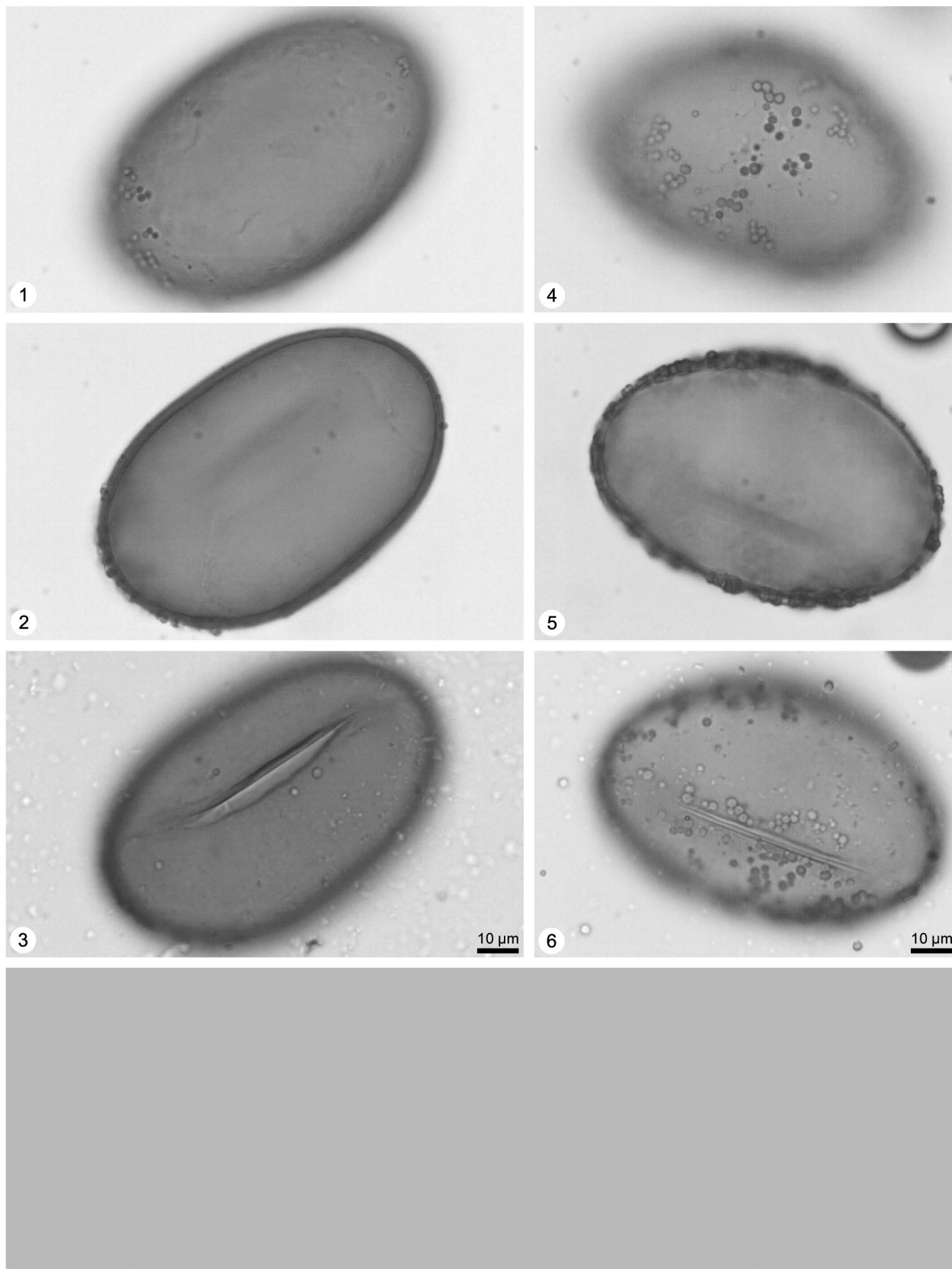
Plate V. Lake Suigetsu Spore Flora: PTERIDOPHYTA - Polypodiopsida - Polypodiales. Polypodiaceae : 1-3 Pyrrosia type, 4-6 Pyrrosia type (1-6 view on distal face, 1-3, 4-6 from high to low focus). Photos/imaging: D. Demske, FUB.
